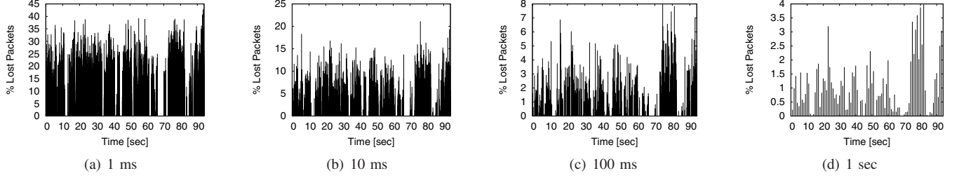
Fig. 2. Packet Loss in fixed windows on multiple timescales
