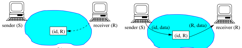
Figure 1: (a) i3 's API. Example illustrating communication between two nodes. (b) The receiver R inserts trigger (id, R) . (c) The sender sends packet (id, data) .
