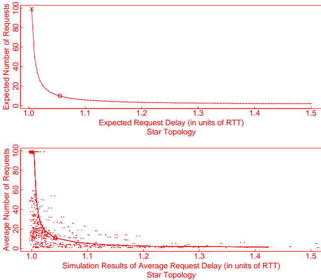
Figure 5: Tradeoff between delay and duplicates in a star topology.
