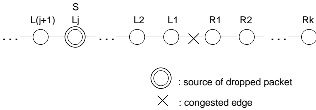
Figure 1: A chain topology.
