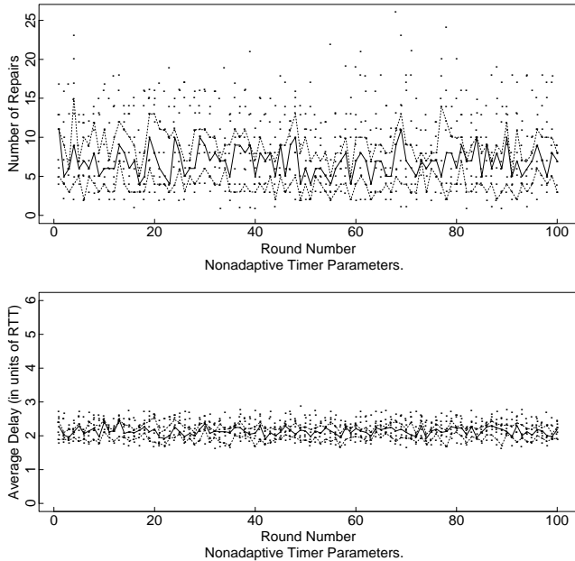
Figure 12: The non-adaptive algorithm.
