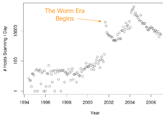
Scan Activity Seen At LBL
