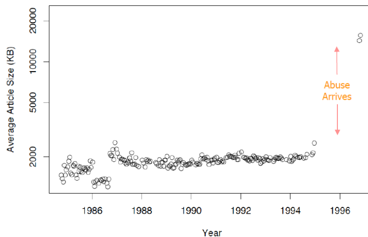
USENET Bulletin Board Traffic Volume
