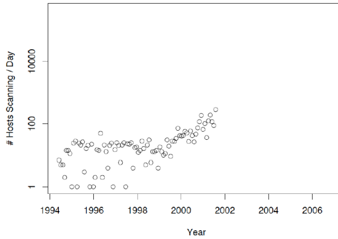
Scan Activity Seen At LBL
