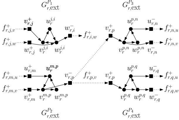
Fig. 4. Extended graphs G_r^P_i, \text{ext} of the paths of service cactus request r of Figure 3. Note that the orientation of edges is reversed, if the virtual edge was reversed in the breadth-first search. This is e.g. the case for the edge (i, j) \in G_r respectively the path P_1 . The flow values f_r^+ , depicted here are used in the Integer Program 3 to induce flows in the extended graphs.
