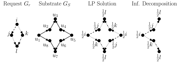
Fig. 6. Example showing that linear relaxations of Integer Program 5 may not be decomposable. The LP solution with x_r = 1 is depicted as follows. Substrate nodes are annotated with the mapping of virtual nodes and \frac{1}{2}i for substrate node u_1 stands for y_{r,i,u_1} = 1/2 . Substrate edges are dashed accordingly to the dash style of the virtual links mapped onto it. All virtual links are mapped with values 1/2 . The dash style of substrate edge (u_1, u_2) therefore implies that z_{r,i,j,u_1,u_2} = 1/2 holds.
