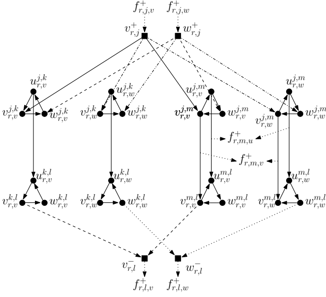
Fig. 5. Extended graph G_{r,ext}^{C_1} of service cactus request r and cycle C_1 depicted in Figure 3. Similar styles of dashed edges incident to the super sources v_{r,j}^+ , w_{r,j}^+ and sinks v_{r,l}^- and w_{r,l}^- indicates that the same amount of flow will be sent along them.
